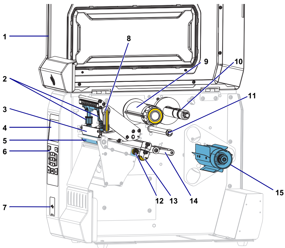
Figure 1 • Printer Components
