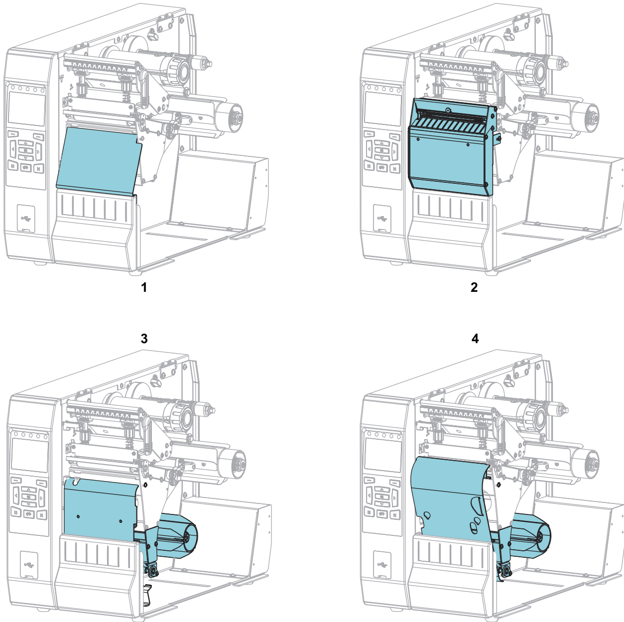
Figure 2 • Printer Options
