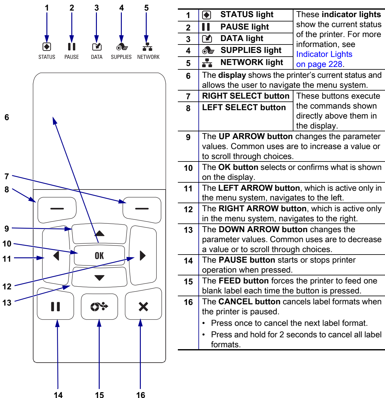
Figure 11 • Control Panel
