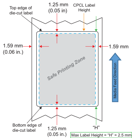
Figure 28 Journal Media
