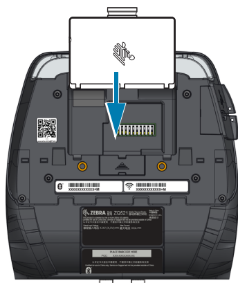
Figure 9 Battery Insertion
