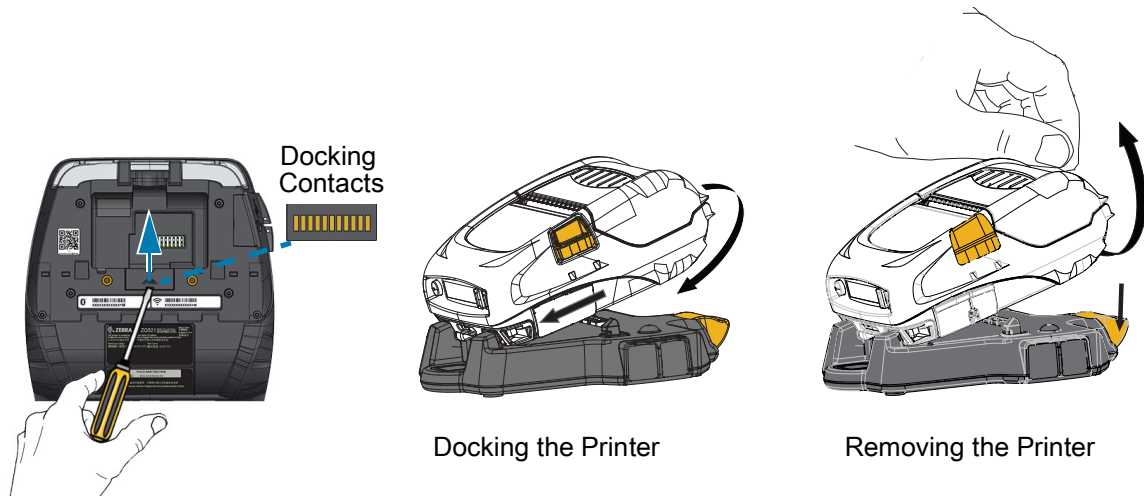
Figure 12 Vehicle Cradle
