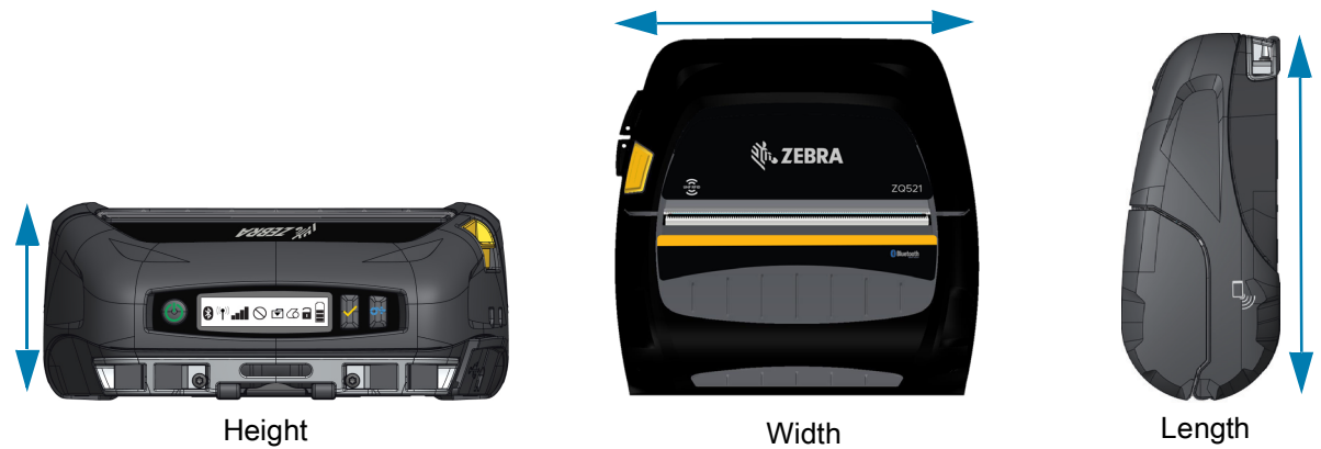
Figure 42 ZQ521 Dimensions
