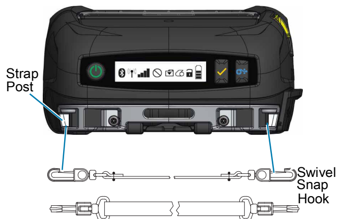
Figure 35 Hand Strap
