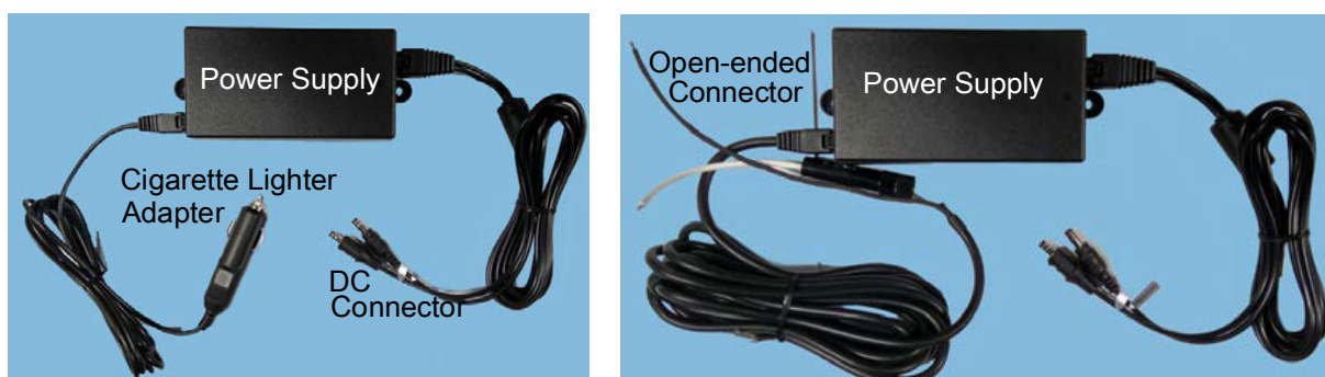
Figure 16 Vehicle Adapters
