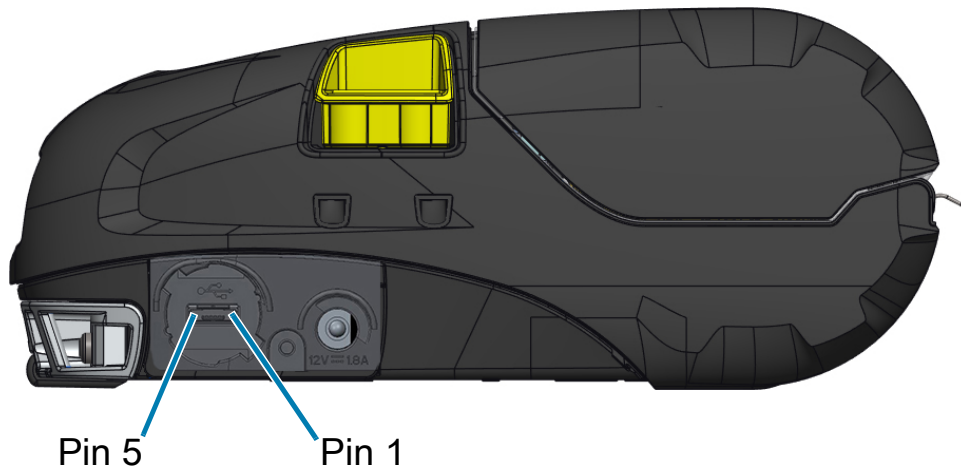
Figure 40 USB Port
