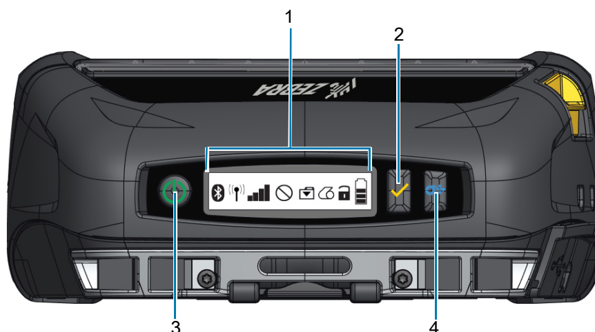
Figure 21 Control Panel
