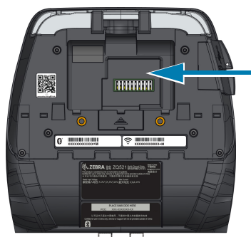
Figure 8 Battery Compartment
